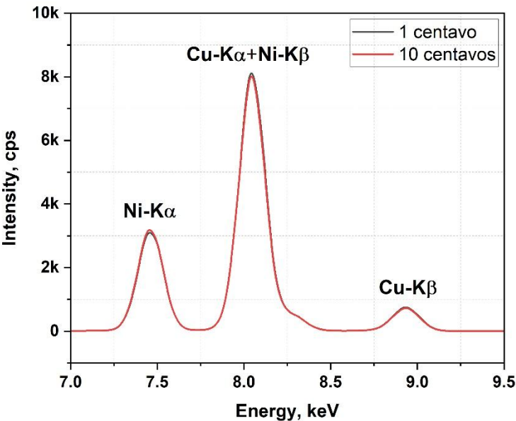
Figure 4: Overlaid average \mu -XRF spectra of the 1 centavo (1988) and 10 centavos (1989) INTUR coins. Spectral similarity indicates alloy equivalence.
